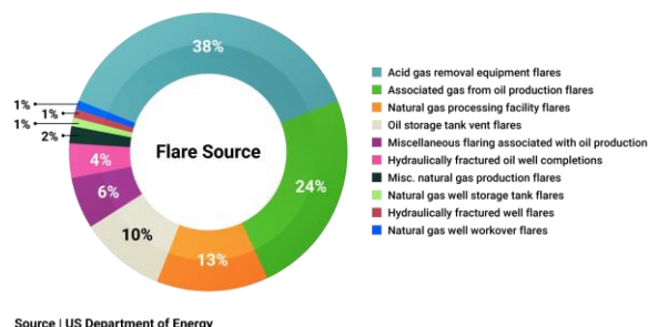
Figure 5 : Gas flaring by sources
