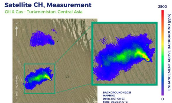
Figure 4 : Methane leakage detected by Satellite
